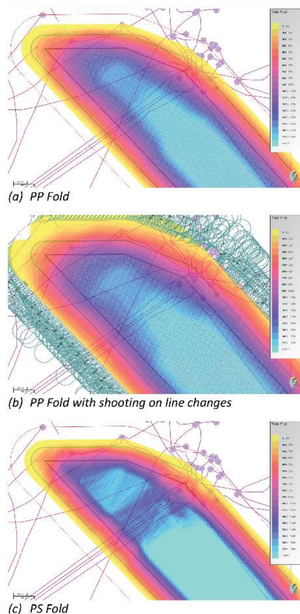
Figure 9 Elevation corrected fold plots for 200m x 200m Rx grid.
