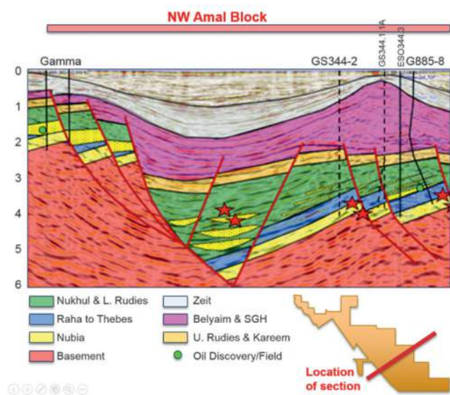
Figure 2 Geologic setting.
