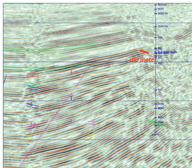
Figure 3 1992 Acquisition + 2017 Processing.
